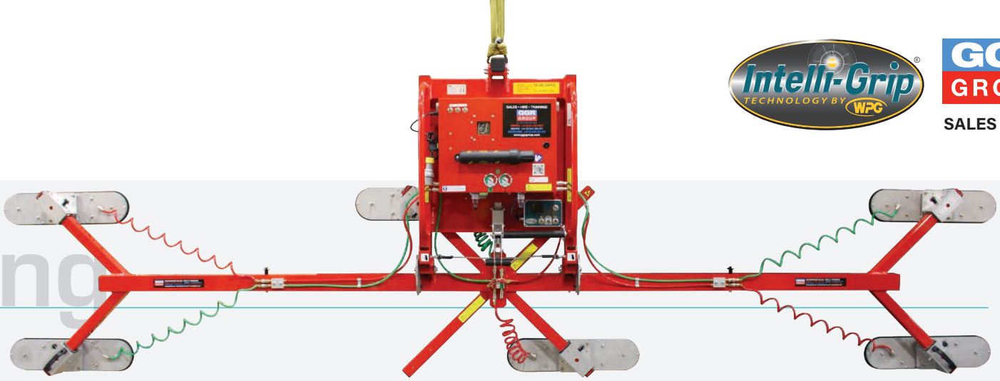
Adjustable lifting bail
